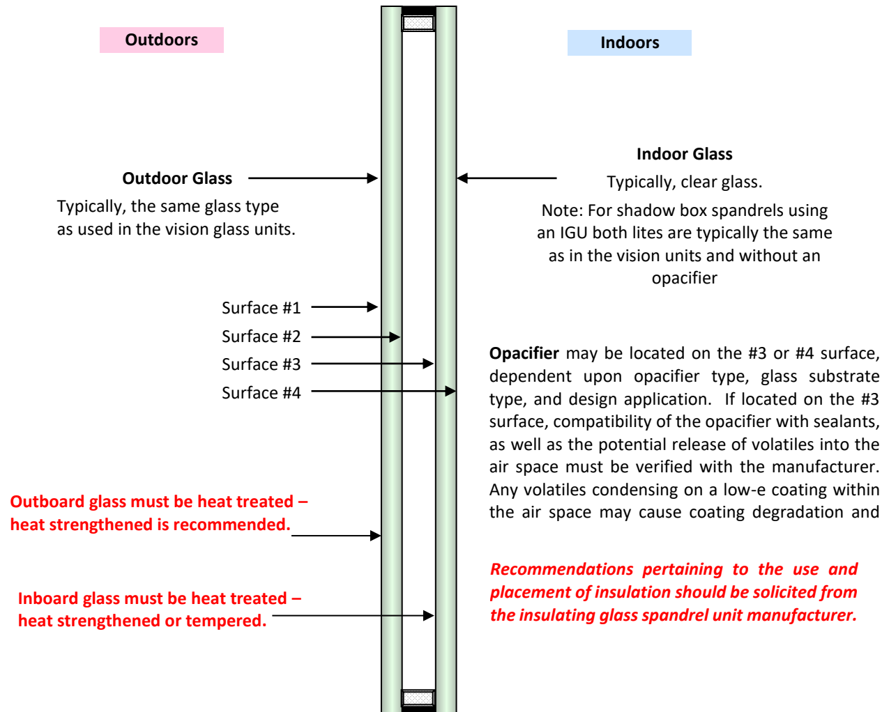
Figure 2 – Insulating Glass Spandrel Unit
